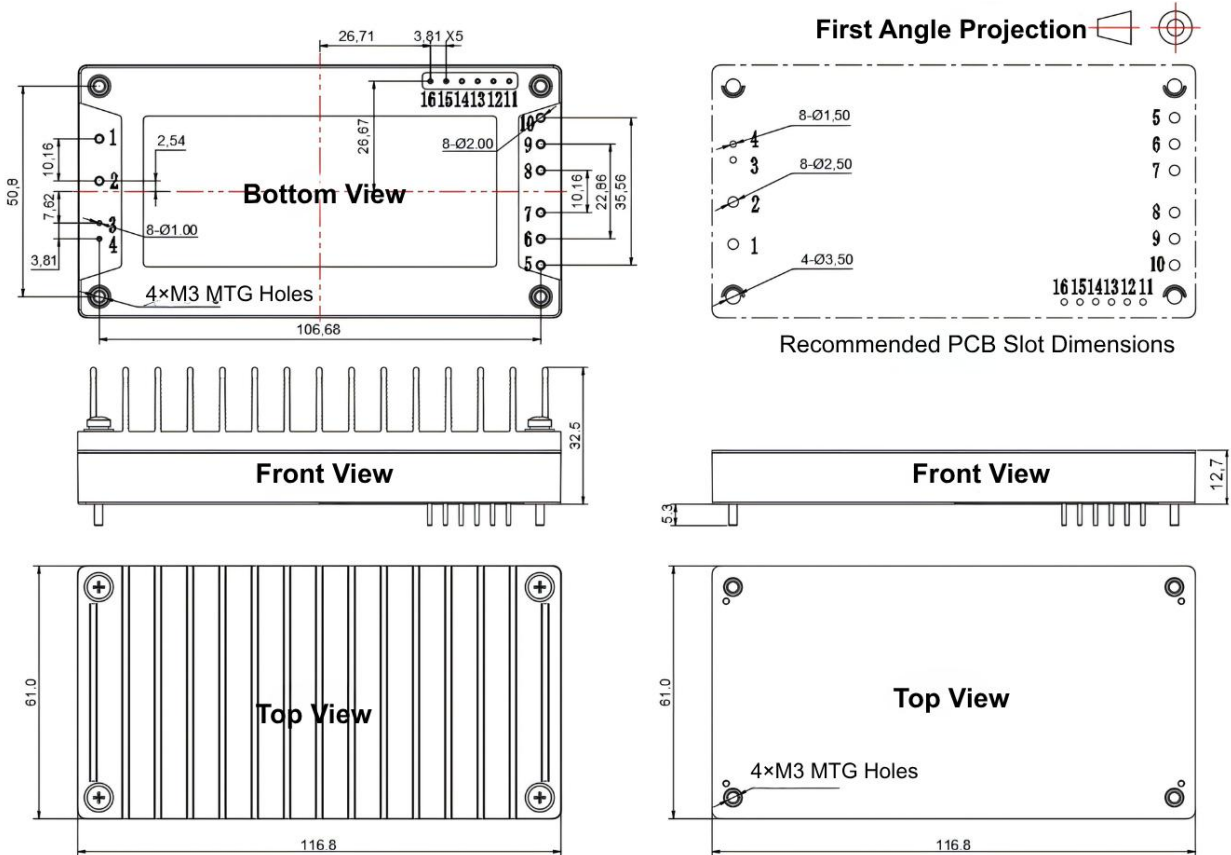
Standard + Heat sink 116.8*61.0*32.50mm
